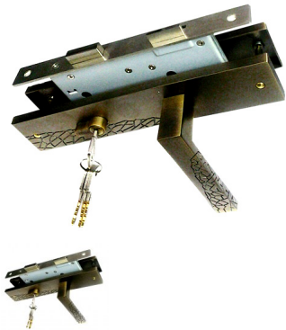
Fealty High Security Lock with 362 MAB handles
